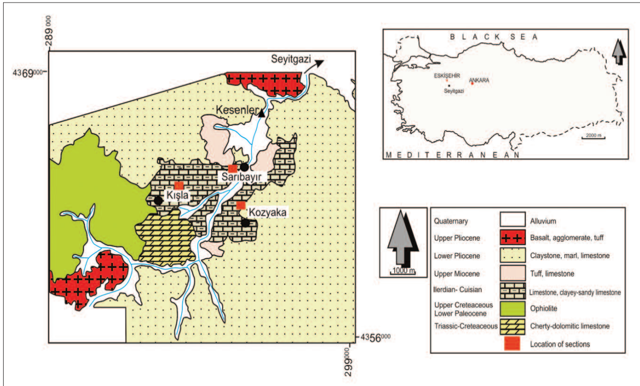
Fig. 1. Geological map of the studied area and location of stratigraphic sections (Geological map modified from Özcan et al., 1989).
