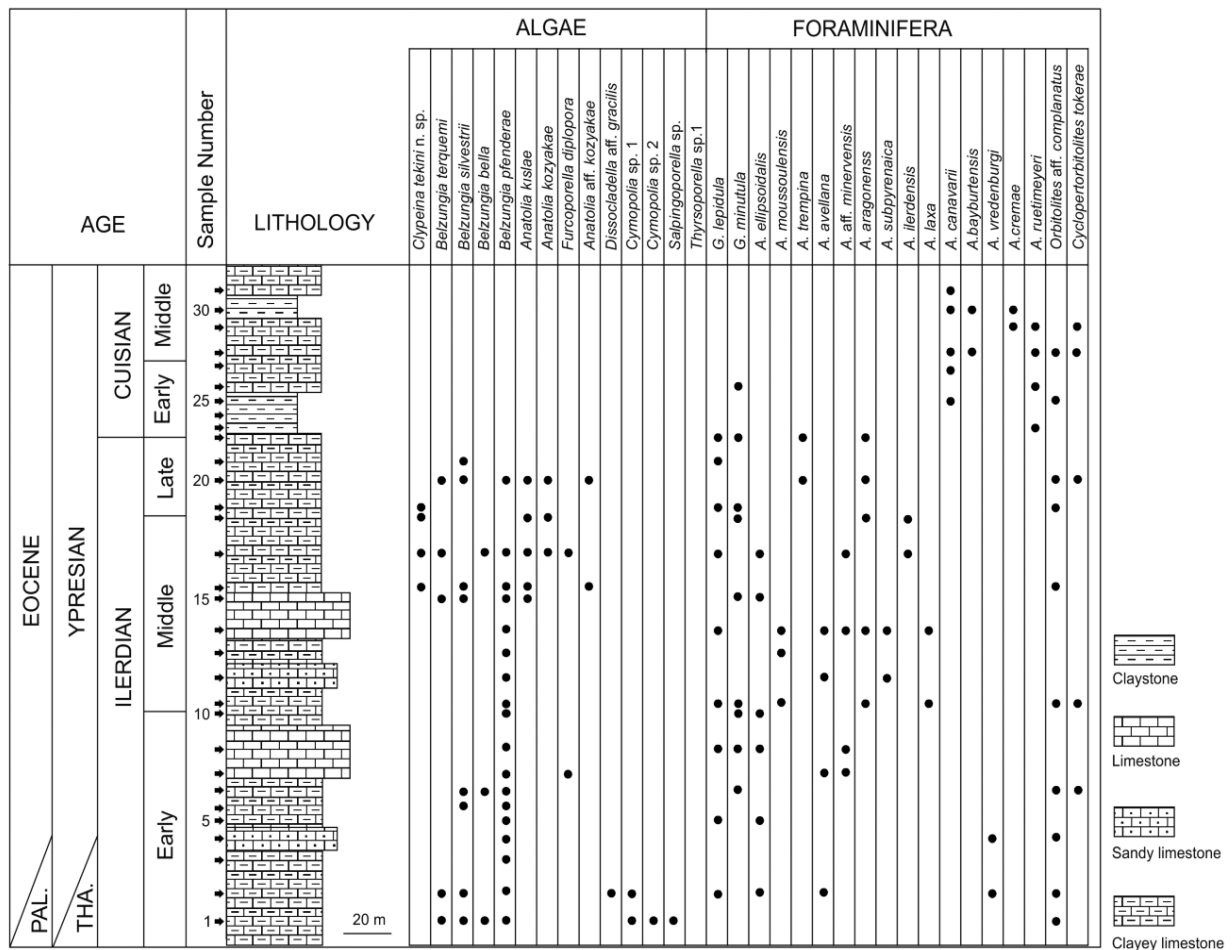
Fig. 2. Stratigraphic distribution of dasycladalean algae and benthic foraminifera in the Sarıbayır section.
